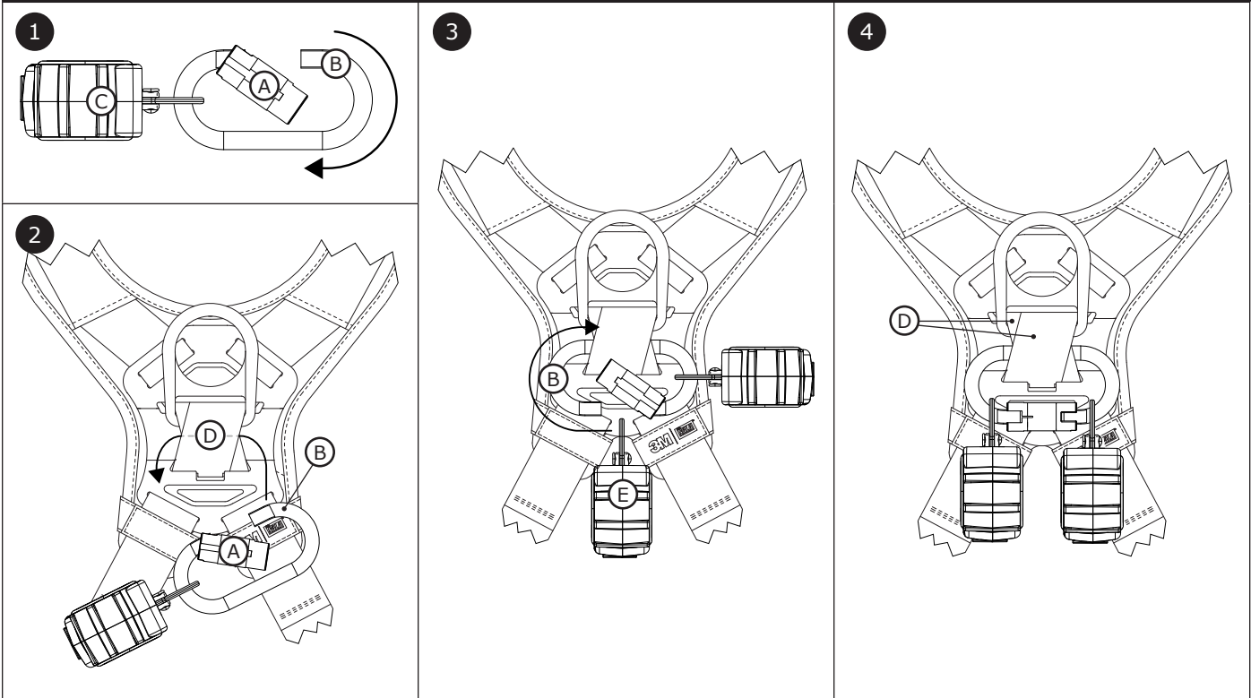
Figure 15 - Carabiner Interface
